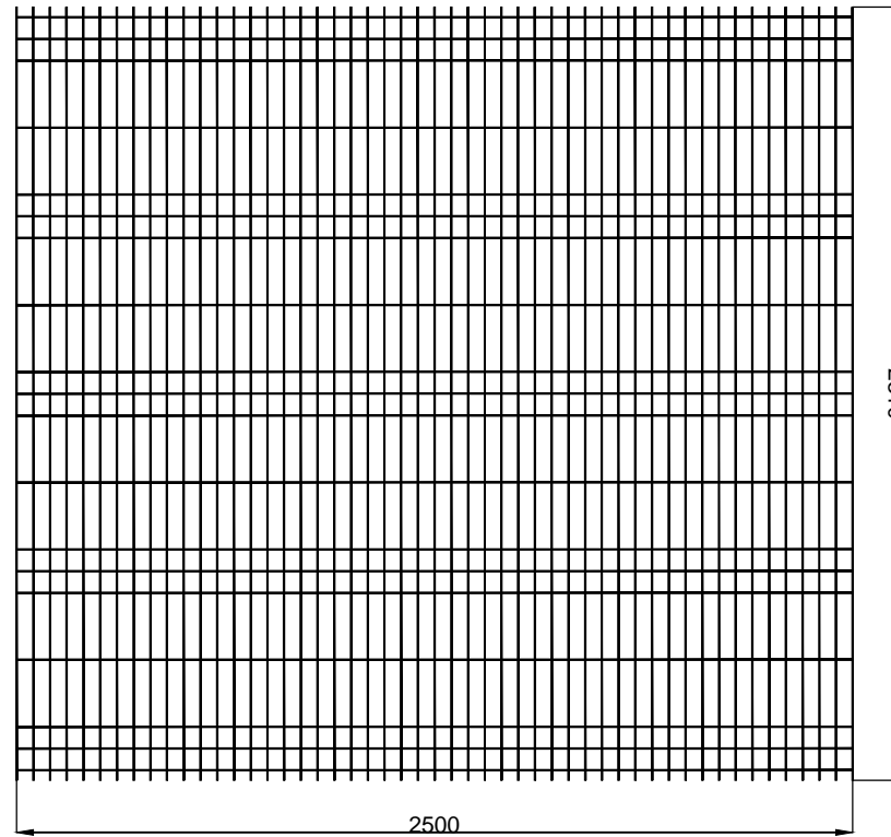
FRONT VIEW - W/O BEND
