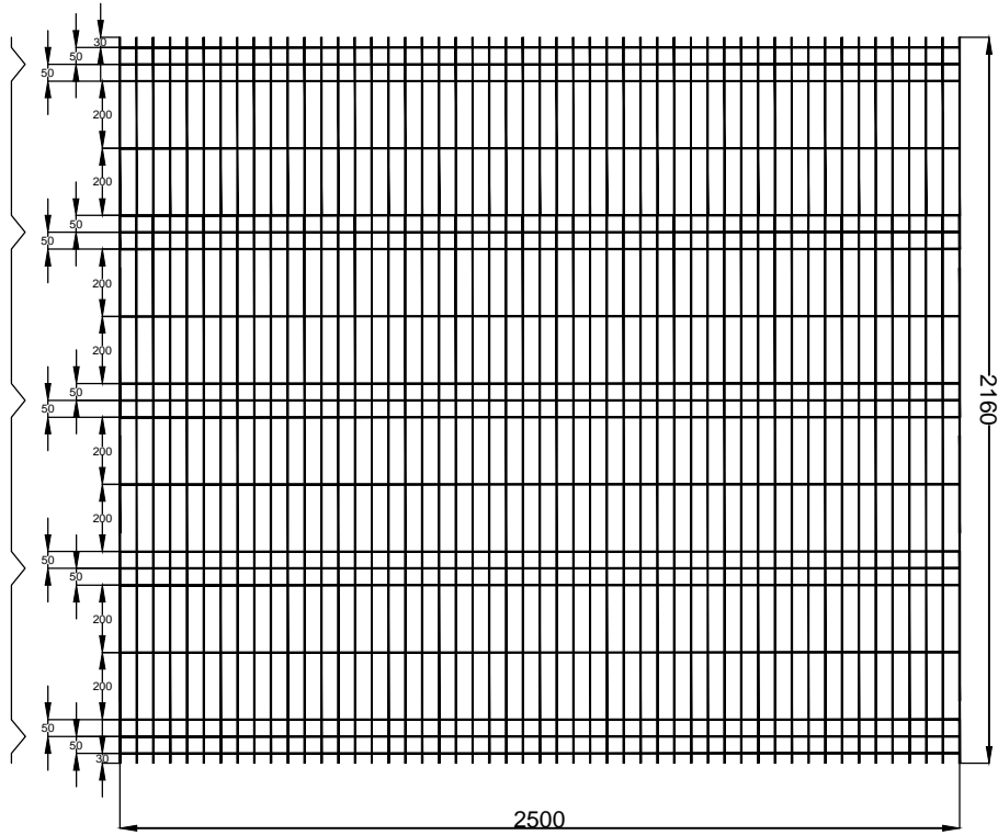
FRONT VIEW - WITH BEND
